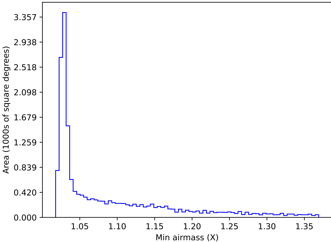
weather_cloudso6v3.4_10yrs WFD i band: Min airmass
