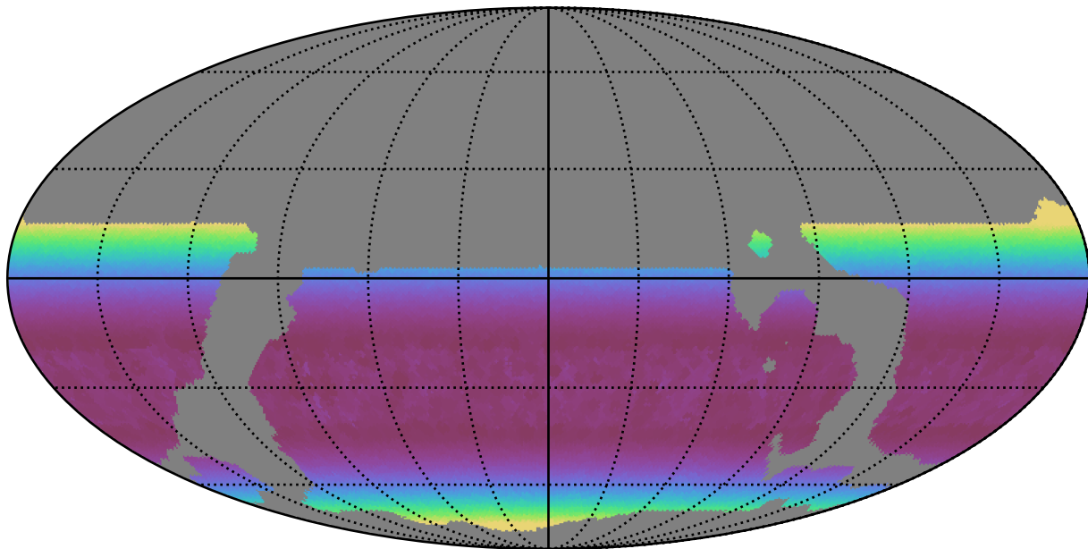
weather_cloudso6v3.4_10yrs WFD g band: Min airmass
