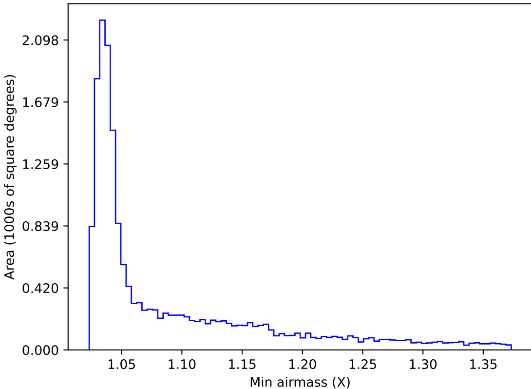
weather_cloudso6v3.4_10yrs WFD g band: Min airmass
