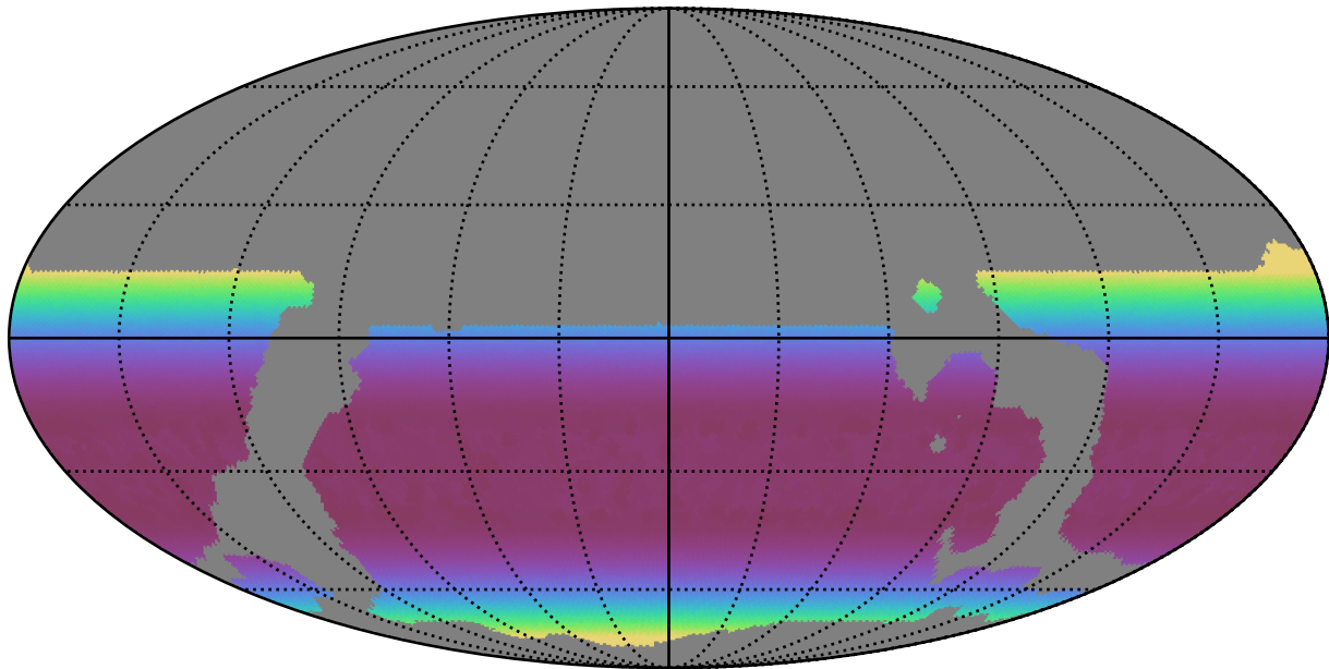
weather_cloudso6v3.4_10yrs WFD all bands: Min airmass
