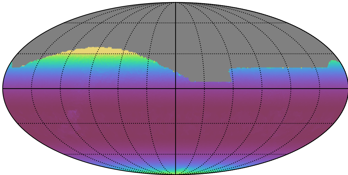
weather_cloudso6v3.4_10yrs All sky z band: Min airmass
