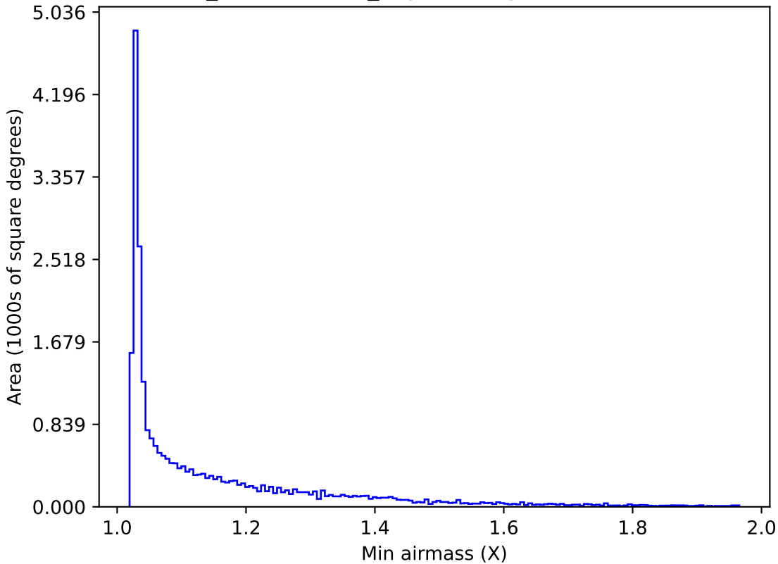
weather_cloudso6v3.4_10yrs All sky z band: Min airmass
