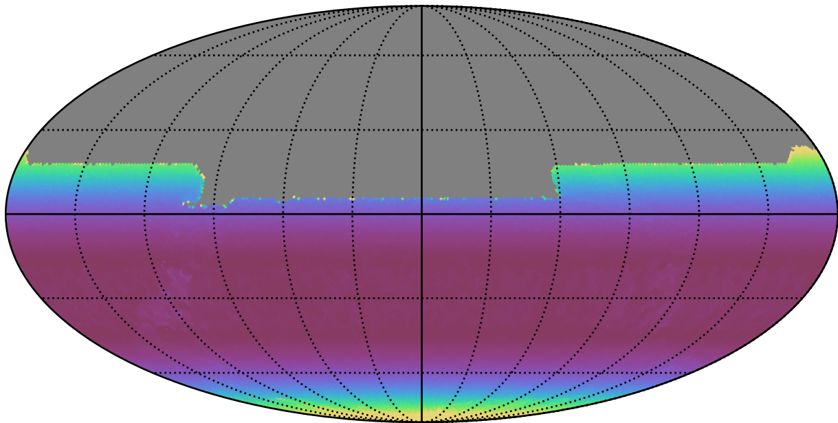
weather_cloudso6v3.4_10yrs All sky y band: Min airmass
