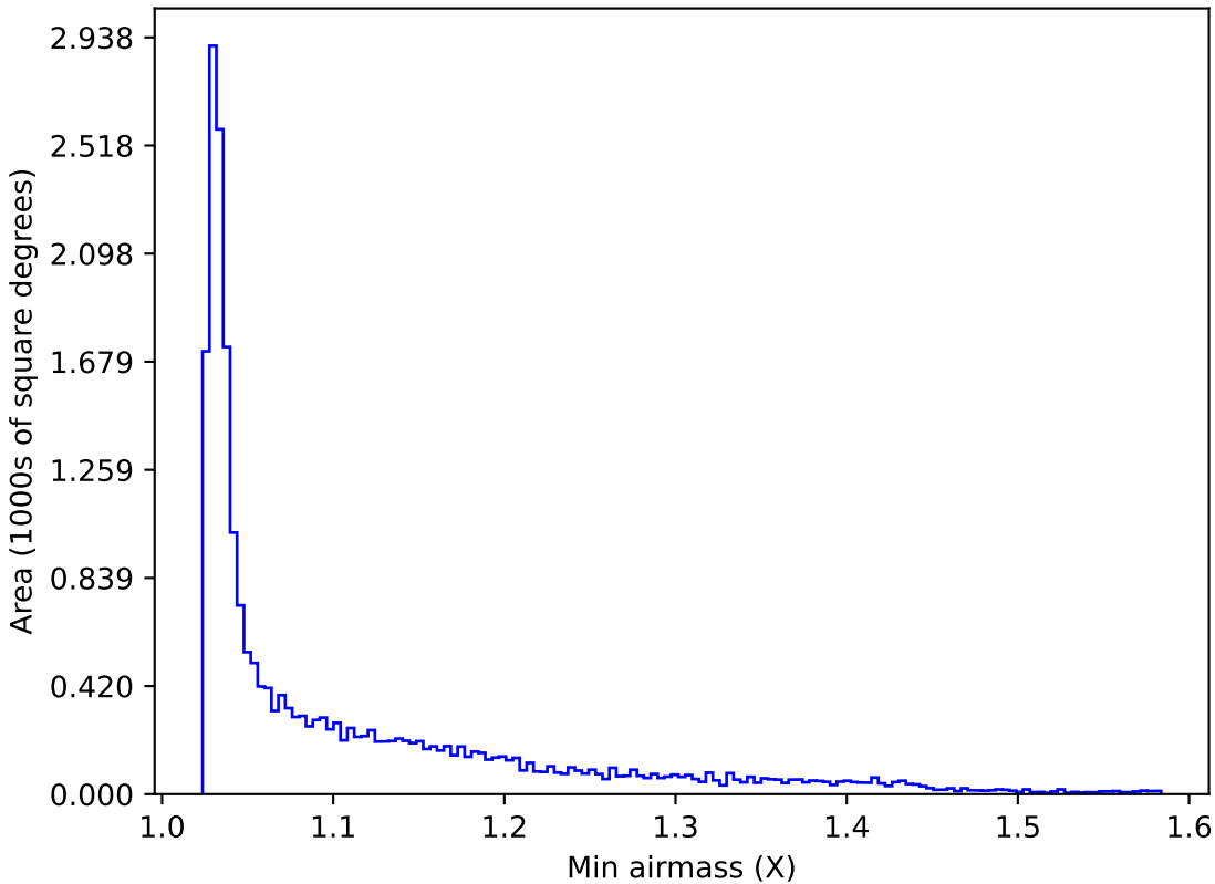
weather_cloudso6v3.4_10yrs All sky y band: Min airmass
