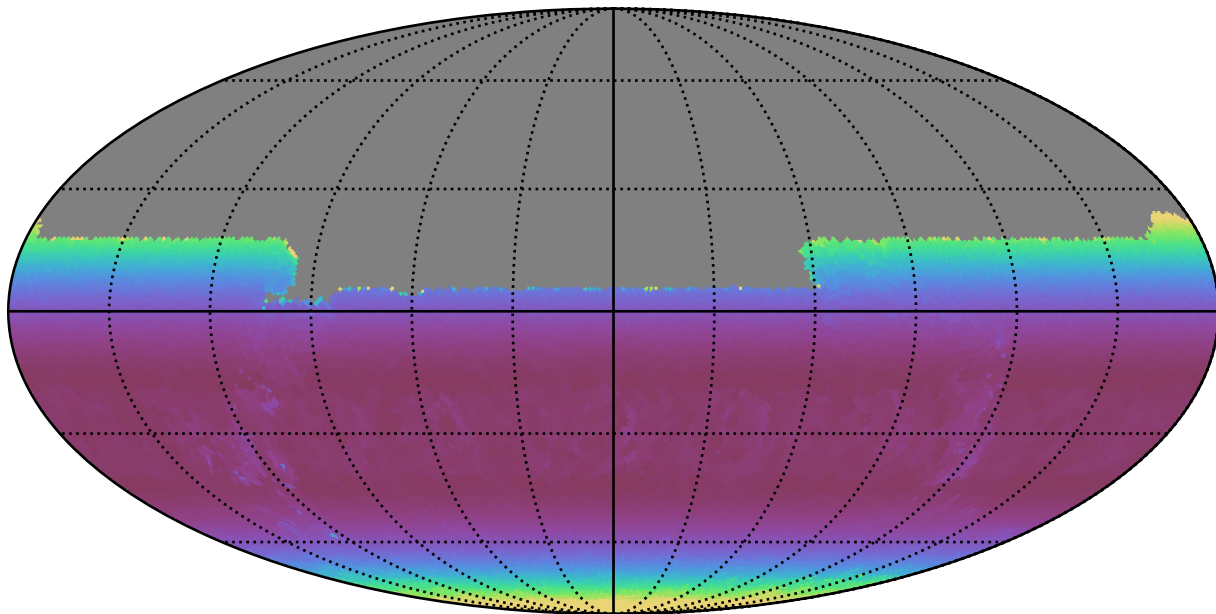
weather_cloudso6v3.4_10yrs All sky u band: Min airmass
