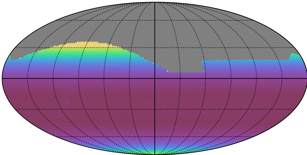
weather_cloudso6v3.4_10yrs All sky i band: Min airmass
