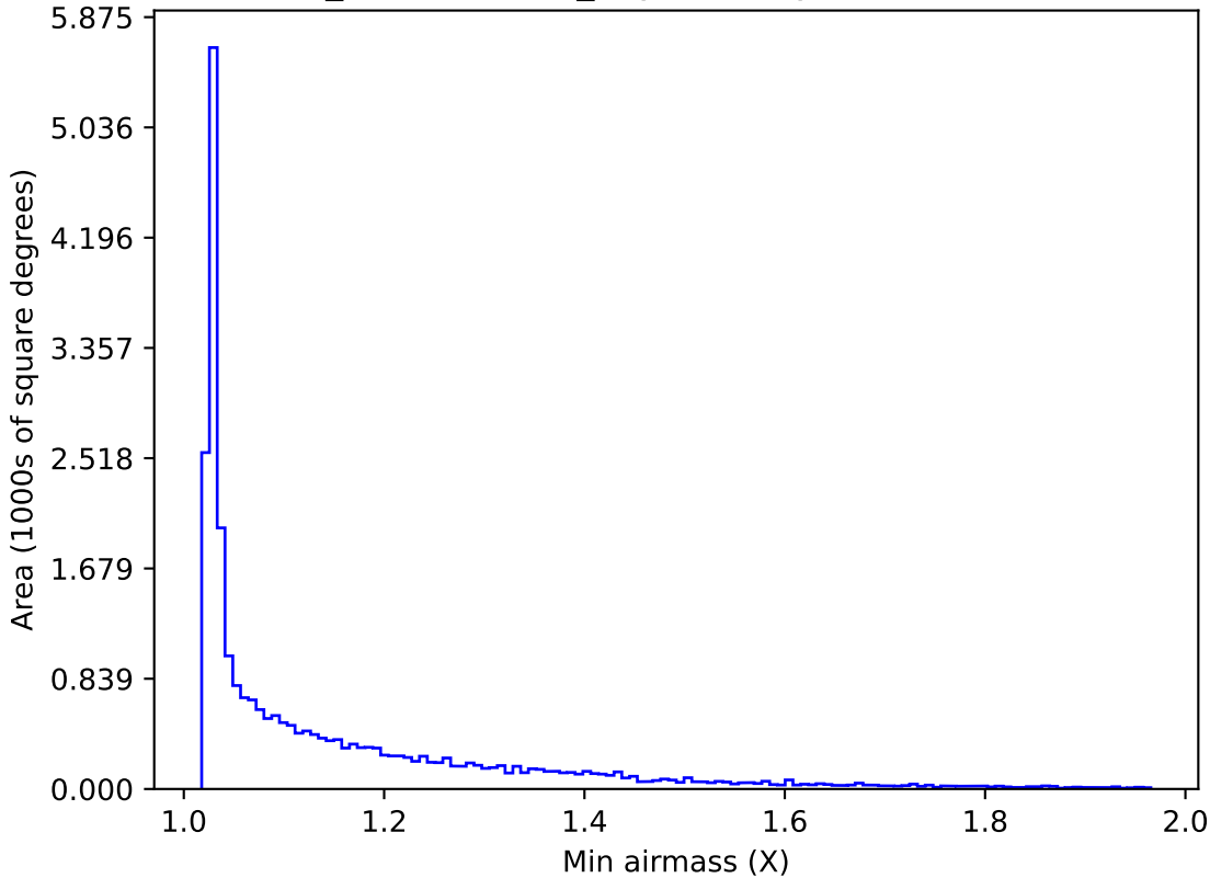
weather_cloudso6v3.4_10yrs All sky i band: Min airmass
