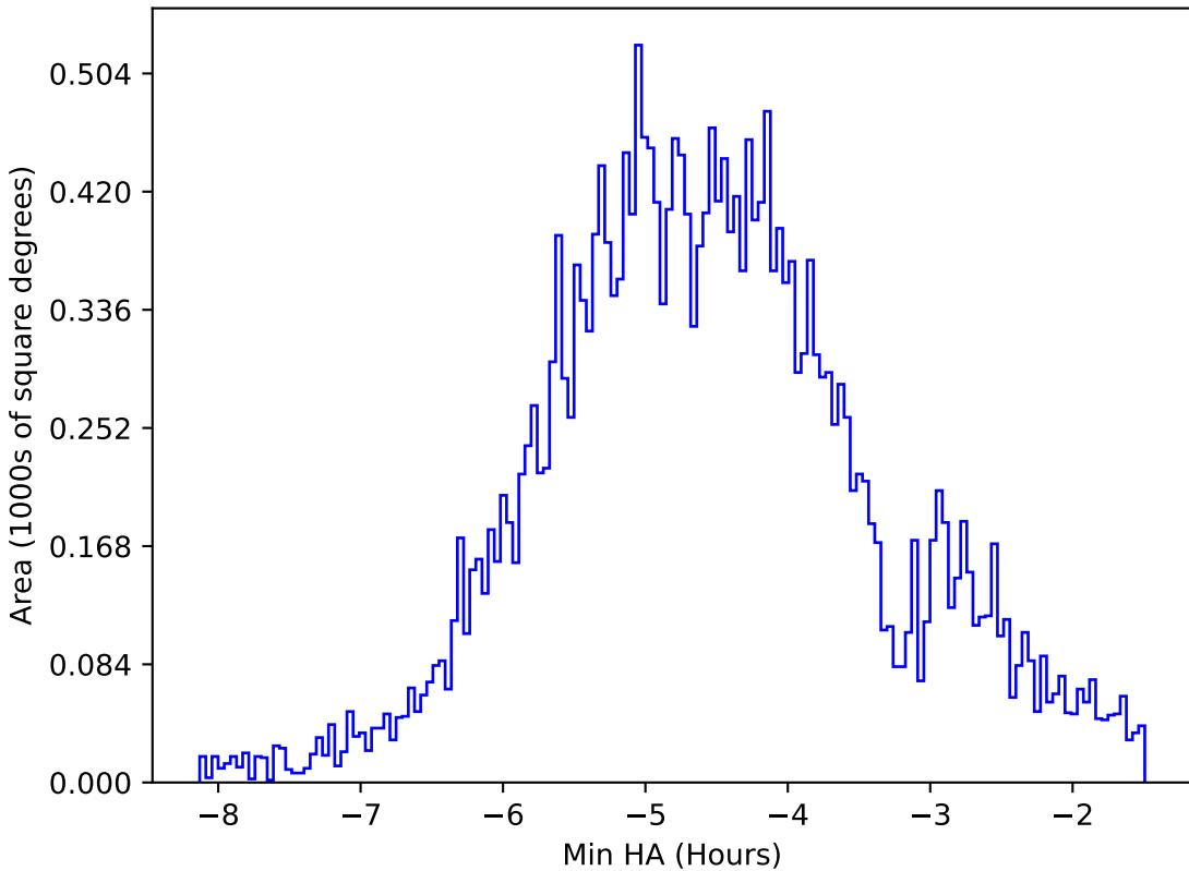
weather_cloudso6v3.4_10yrs All sky all bands: Min HA
