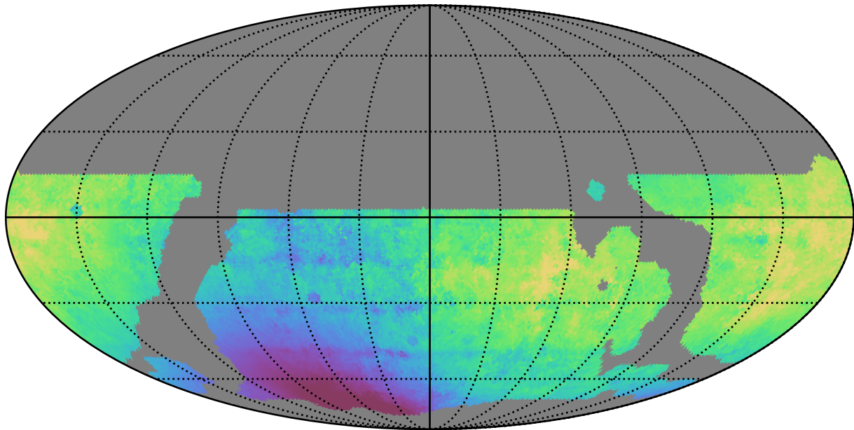
weather_cloudso6v3.4_10yrs WFD z band: Median solarElong
