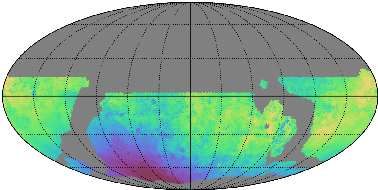
weather_cloudso6v3.4_10yrs WFD u band: Median solarElong
