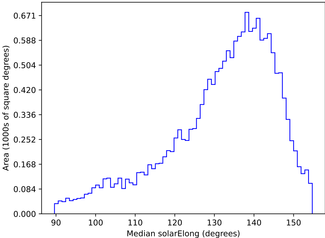
weather_cloudso6v3.4_10yrs WFD u band: Median solarElong
