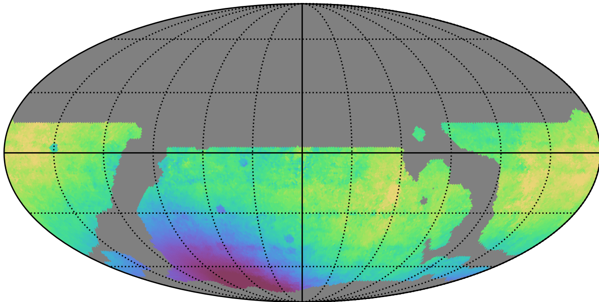
weather_cloudso6v3.4_10yrs WFD r band: Median solarElong
