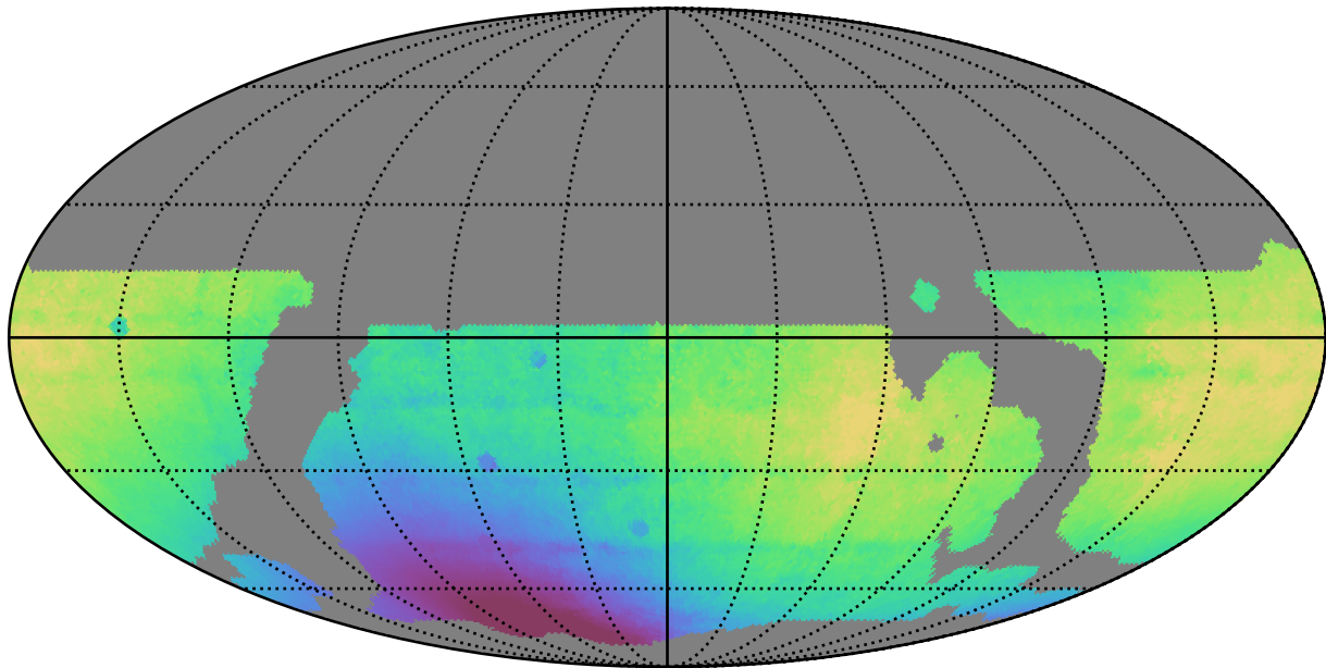
weather_cloudso6v3.4_10yrs WFD all bands: Median solarElong
