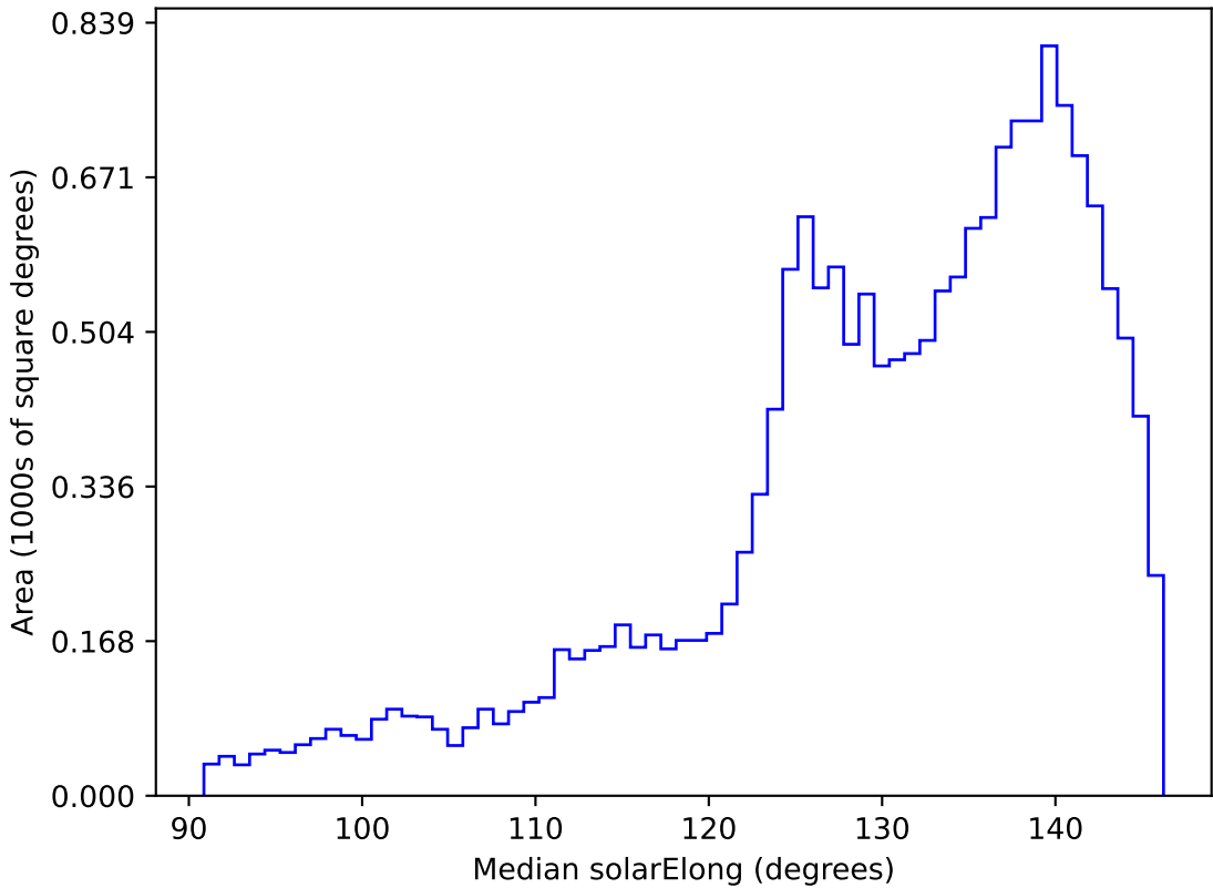
weather_cloudso6v3.4_10yrs WFD all bands: Median solarElong
