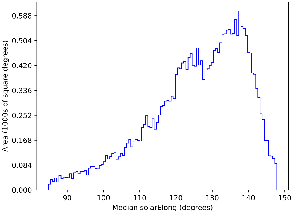
weather_cloudso6v3.4_10yrs All sky z band: Median solarElong
