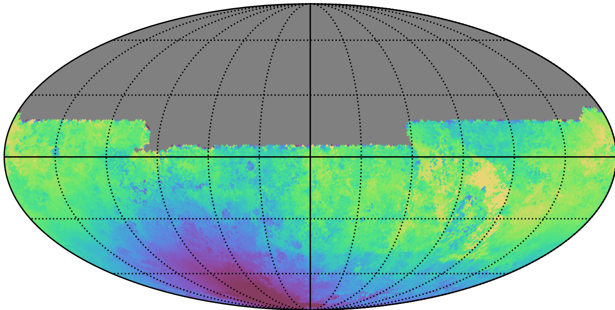
weather_cloudso6v3.4_10yrs All sky u band: Median solarElong
