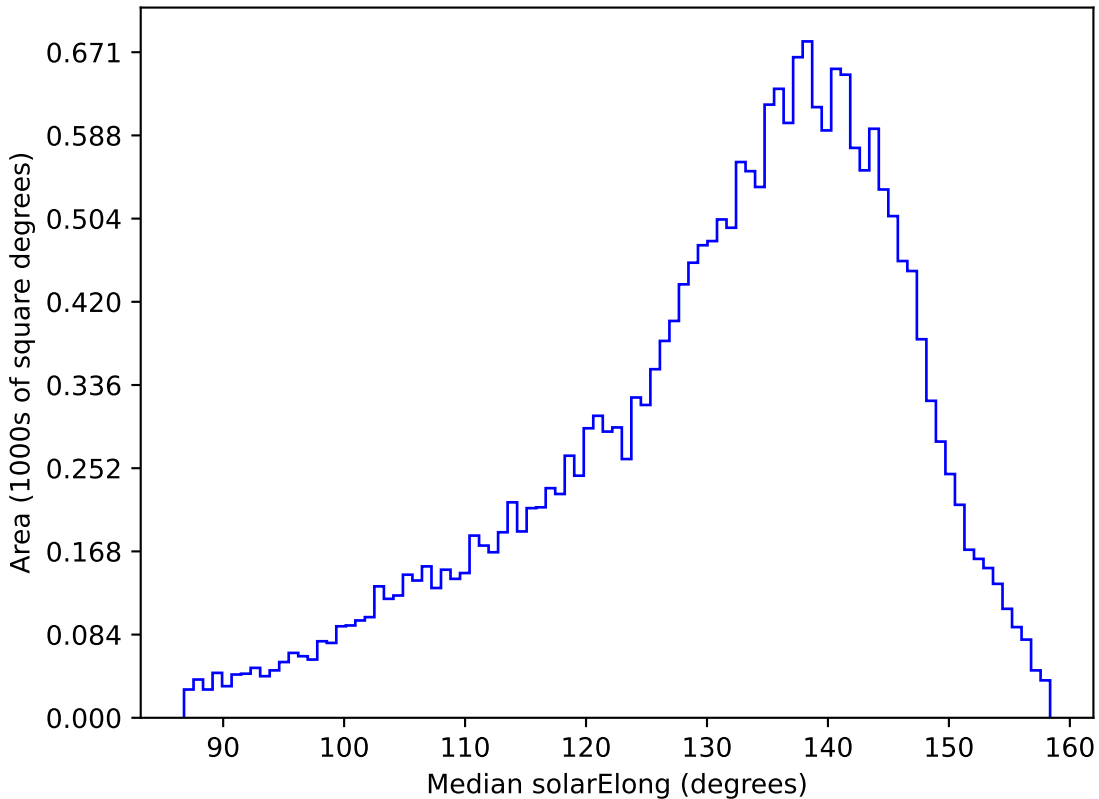
weather_cloudso6v3.4_10yrs All sky u band: Median solarElong
