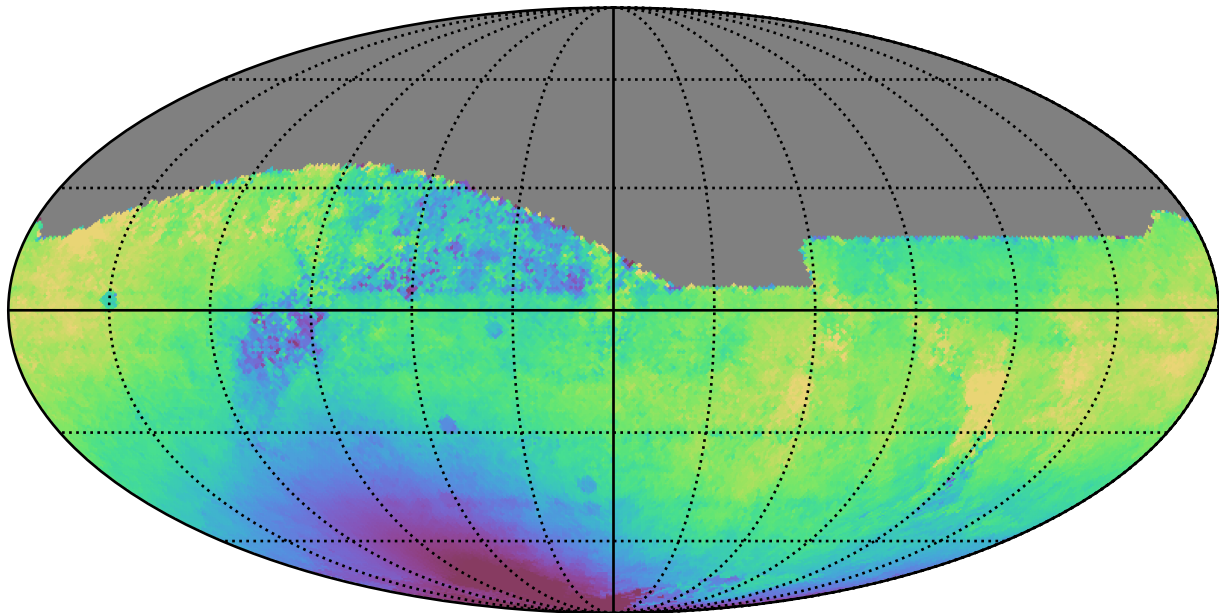
weather_cloudso6v3.4_10yrs All sky r band: Median solarElong
