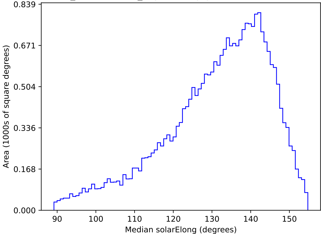
weather_cloudso6v3.4_10yrs All sky g band: Median solarElong
