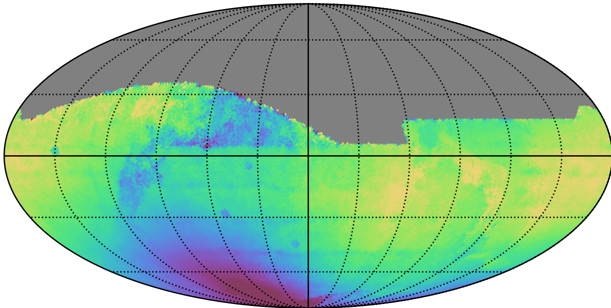
weather_cloudso6v3.4_10yrs All sky all bands: Median solarElong
