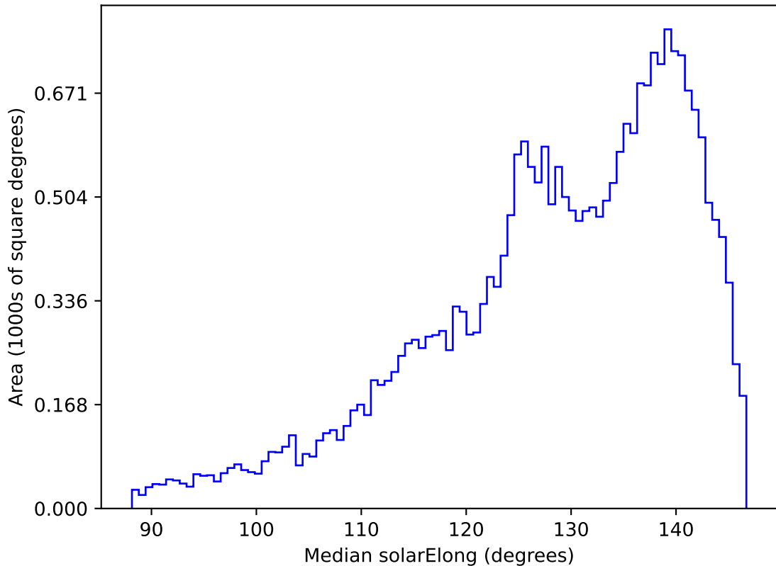
weather_cloudso6v3.4_10yrs All sky all bands: Median solarElong
