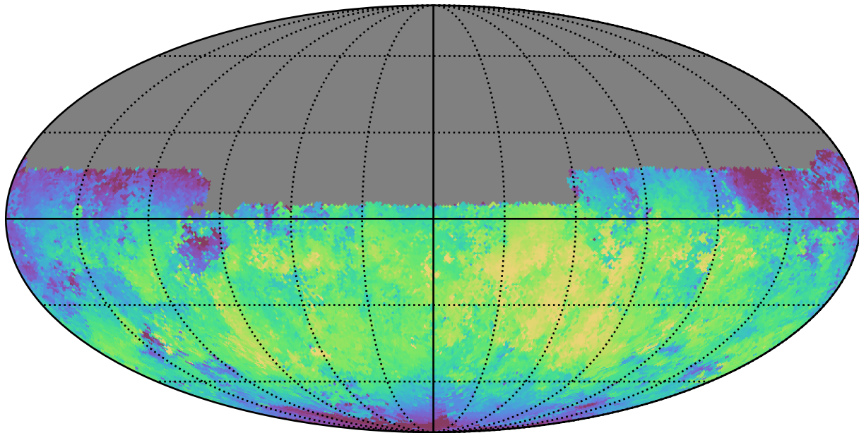
weather_cloudso6v3.4_10yrs Yr 1 y band: Median skyBrightness
