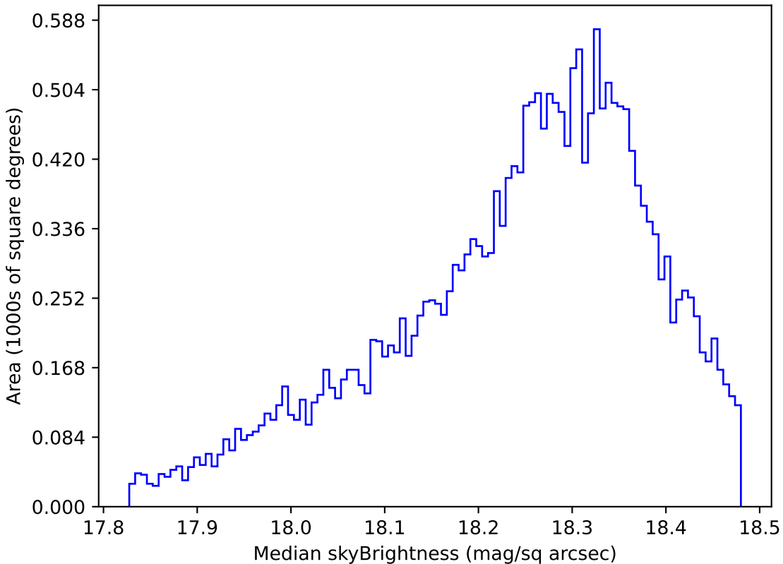
weather_cloudso6v3.4_10yrs Yr 1 y band: Median skyBrightness
