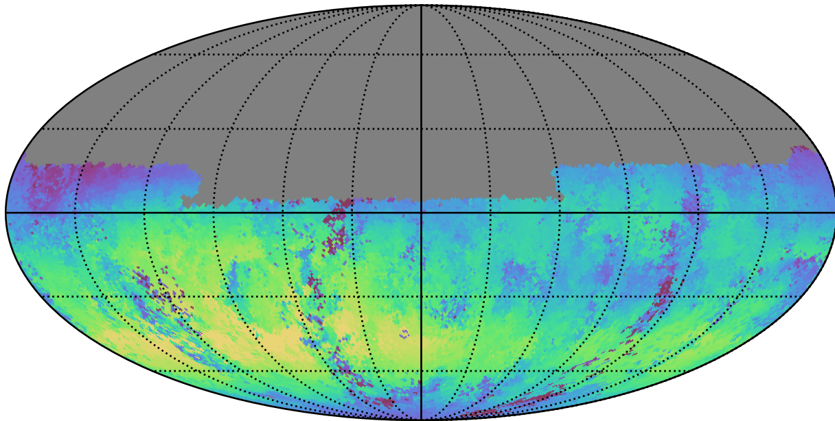
weather_cloudso6v3.4_10yrs Yr 1 u band: Median skyBrightness
