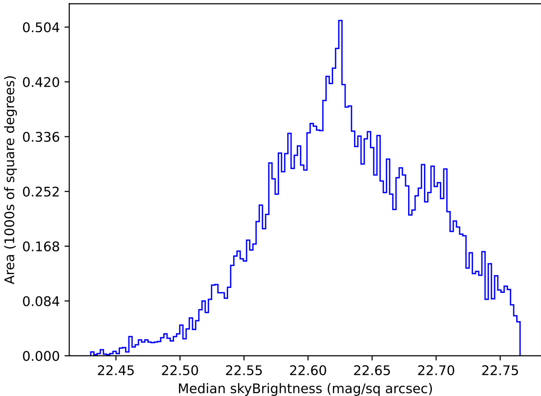
weather_cloudso6v3.4_10yrs Yr 1 u band: Median skyBrightness
