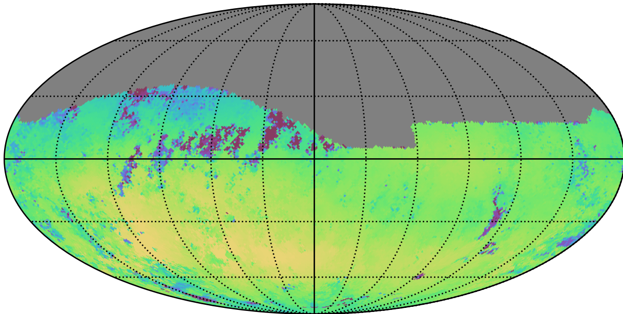
weather_cloudso6v3.4_10yrs Yr 1 r band: Median skyBrightness
