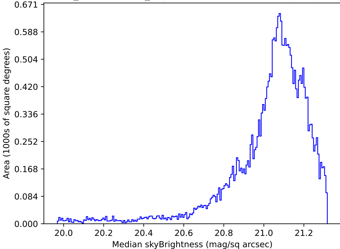
weather_cloudso6v3.4_10yrs Yr 1 r band: Median skyBrightness
