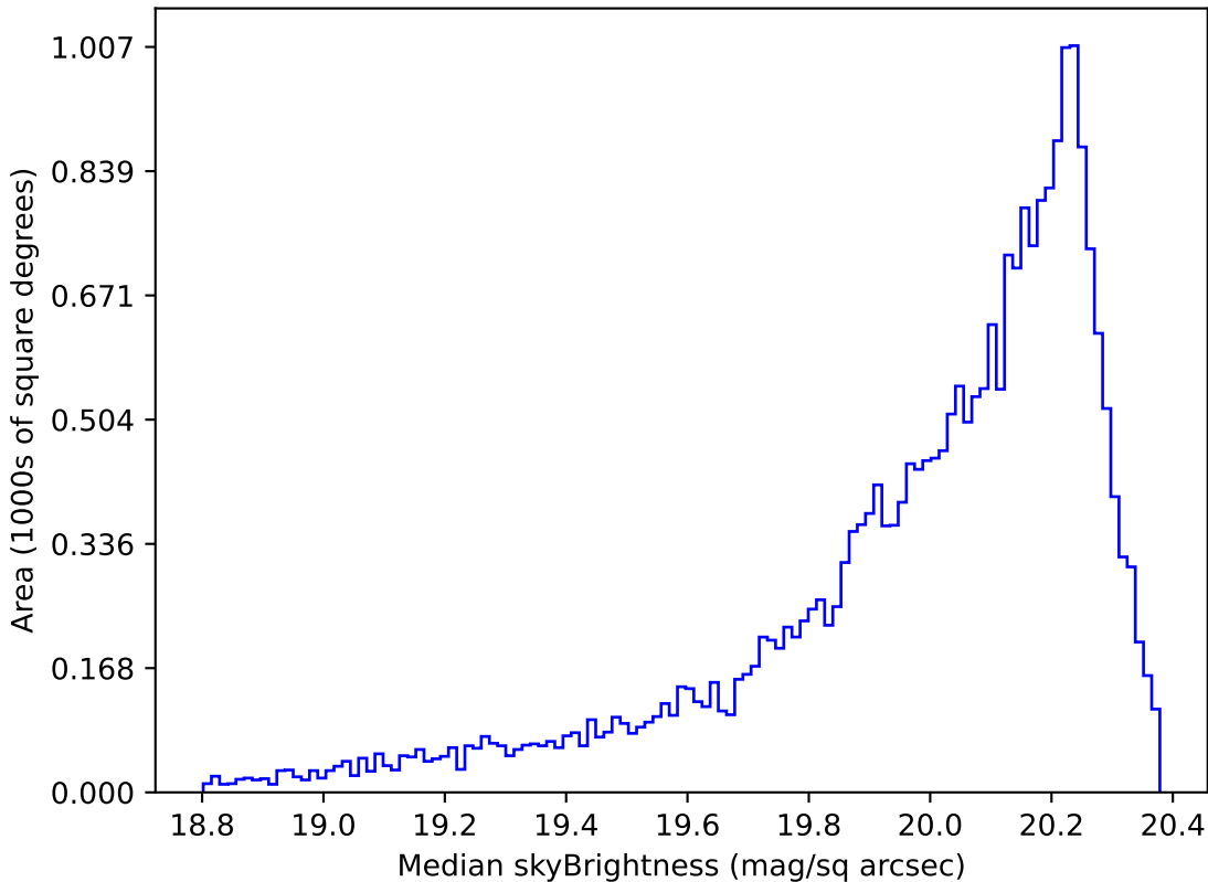
weather_cloudso6v3.4_10yrs Yr 1 i band: Median skyBrightness
