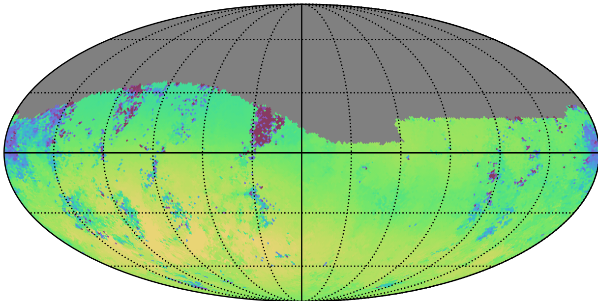
weather_cloudso6v3.4_10yrs Yr 1 g band: Median skyBrightness
