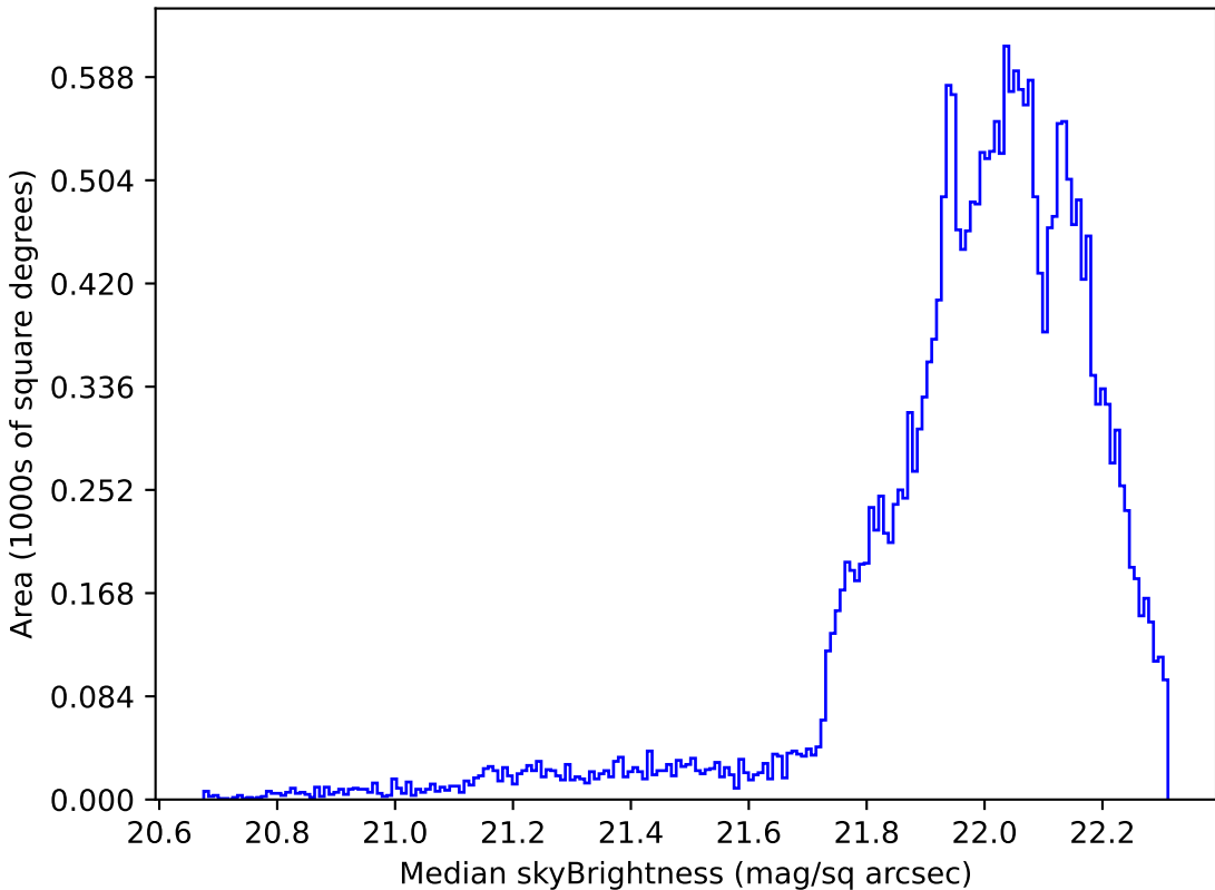
weather_cloudso6v3.4_10yrs Yr 1 g band: Median skyBrightness
