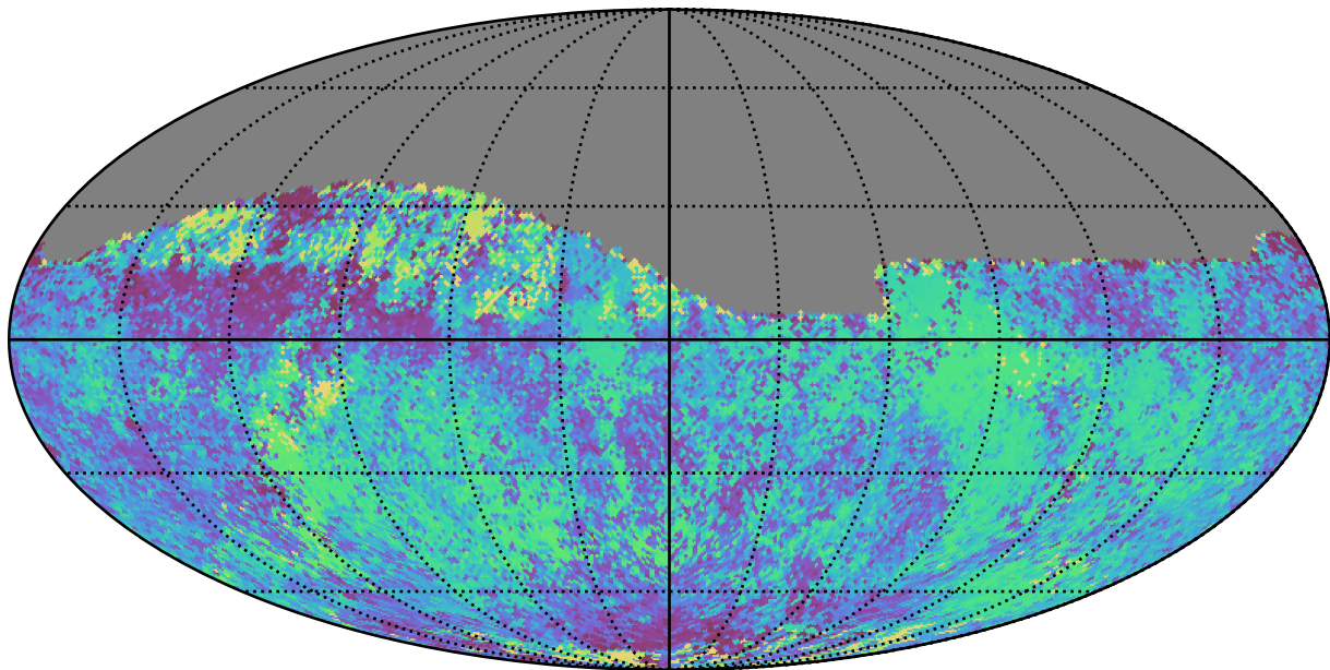
weather_cloudso6v3.4_10yrs Yr 1 all bands: Median skyBrightness
