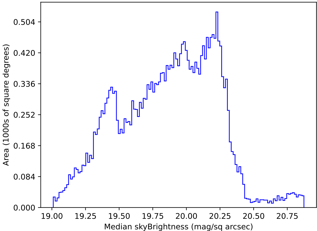
weather_cloudso6v3.4_10yrs Yr 1 all bands: Median skyBrightness
