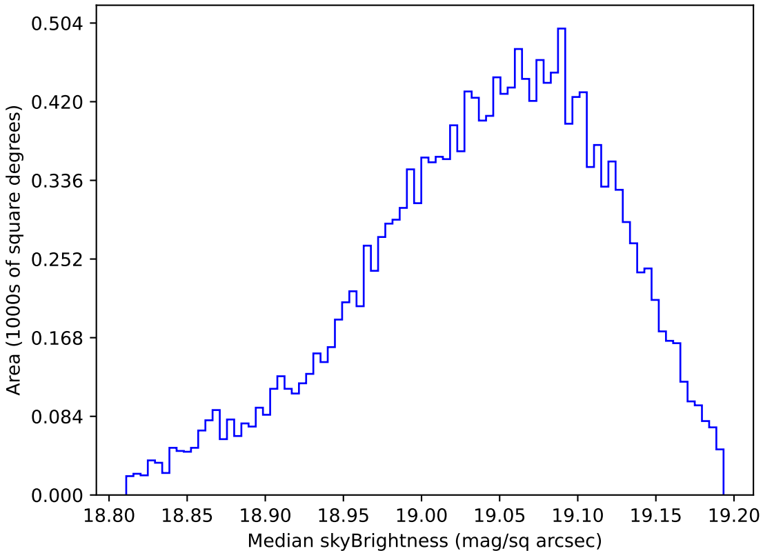
weather_cloudso6v3.4_10yrs WFD z band: Median skyBrightness
