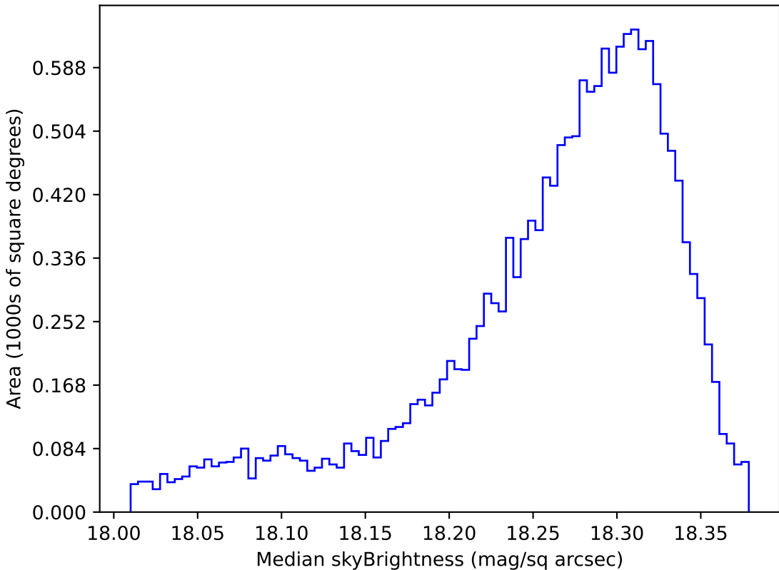
weather_cloudso6v3.4_10yrs WFD y band: Median skyBrightness
