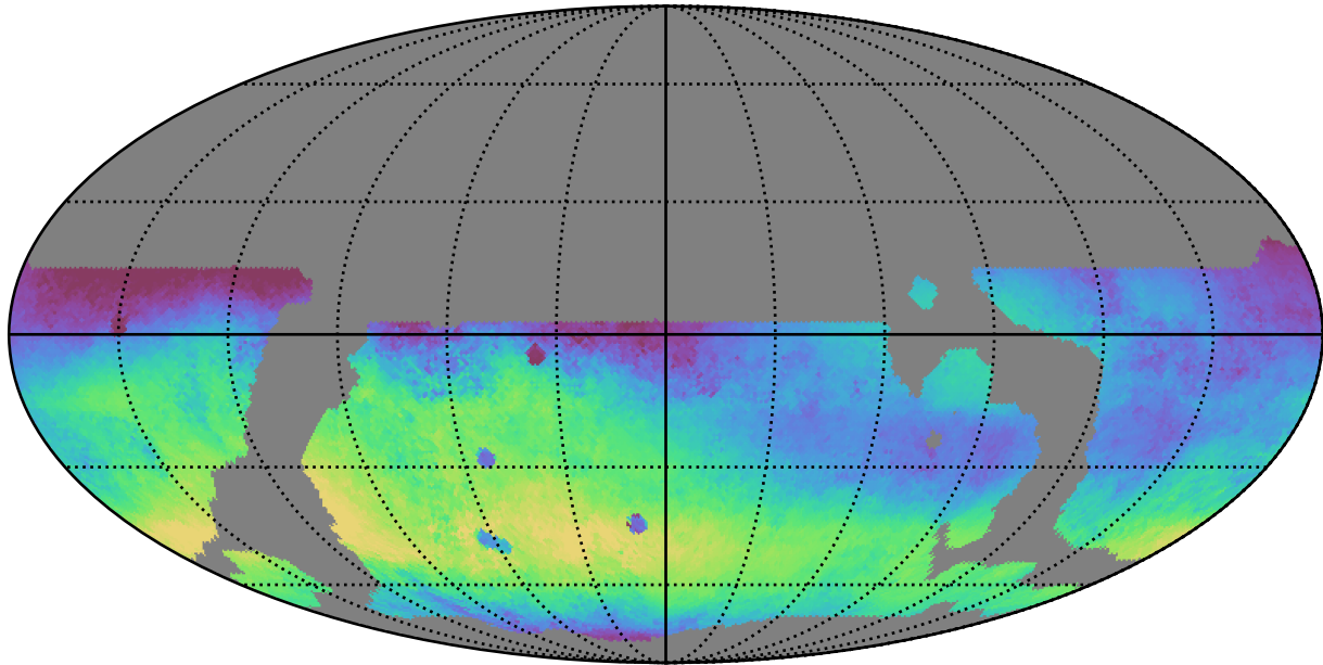
weather_cloudso6v3.4_10yrs WFD r band: Median skyBrightness
