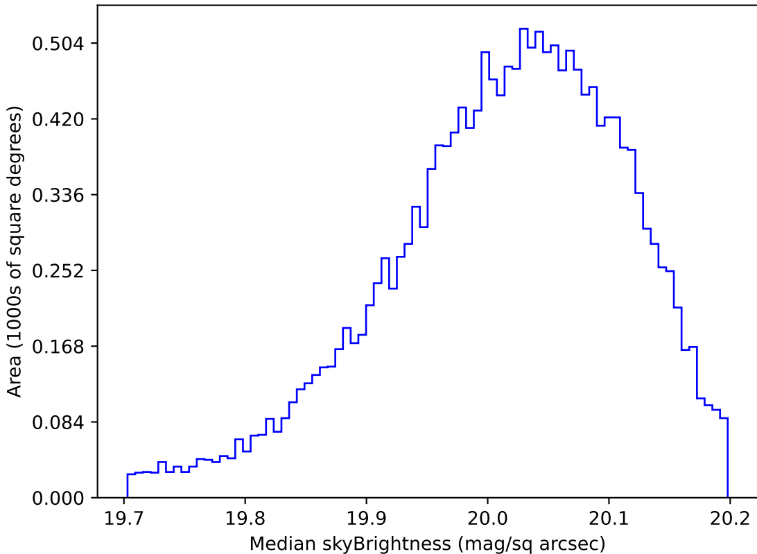
weather_cloudso6v3.4_10yrs WFD i band: Median skyBrightness
