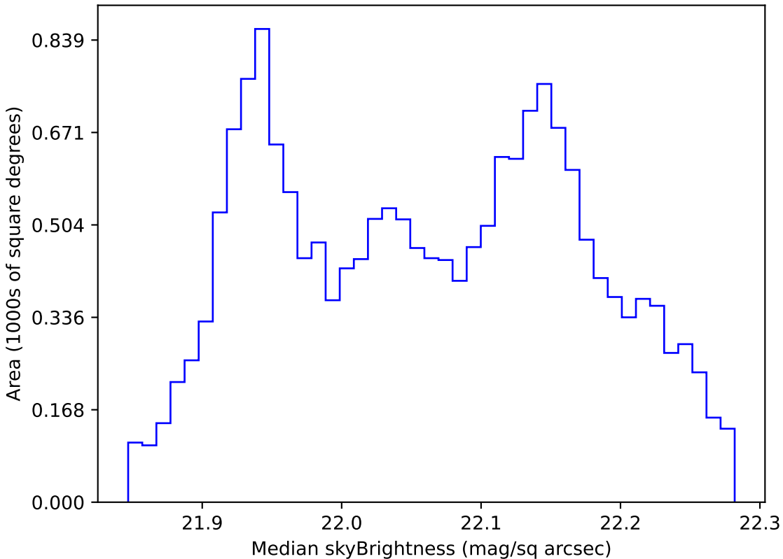
weather_cloudso6v3.4_10yrs WFD g band: Median skyBrightness
