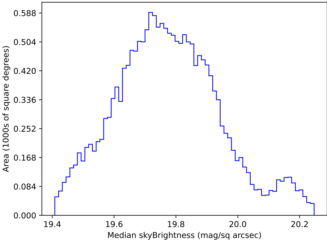
weather_cloudso6v3.4_10yrs WFD all bands: Median skyBrightness
