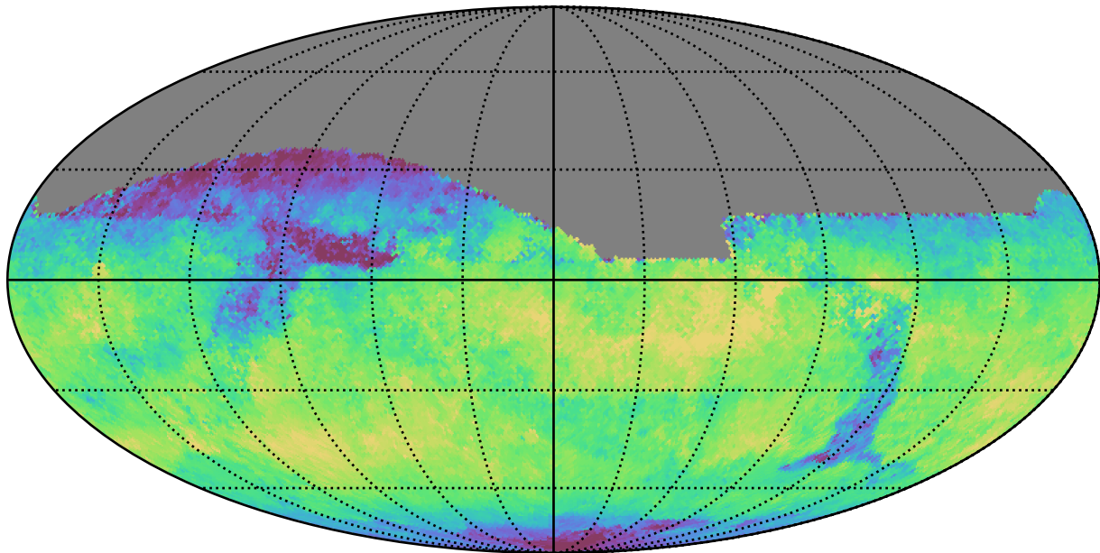
weather_cloudso6v3.4_10yrs All sky z band: Median skyBrightness
