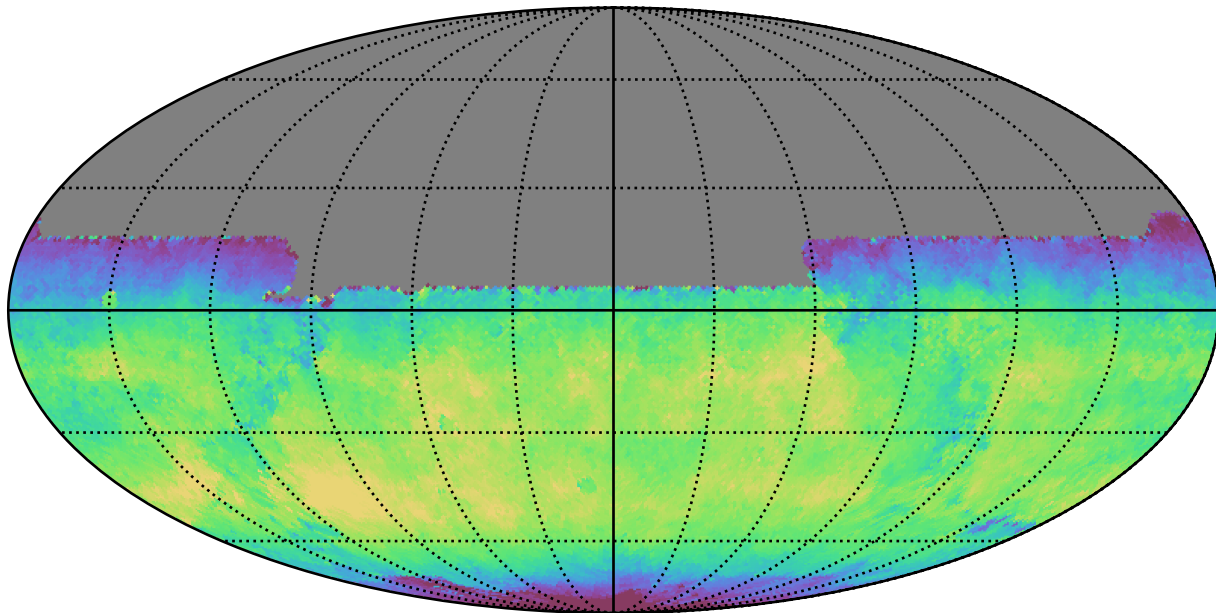
weather_cloudso6v3.4_10yrs All sky y band: Median skyBrightness
