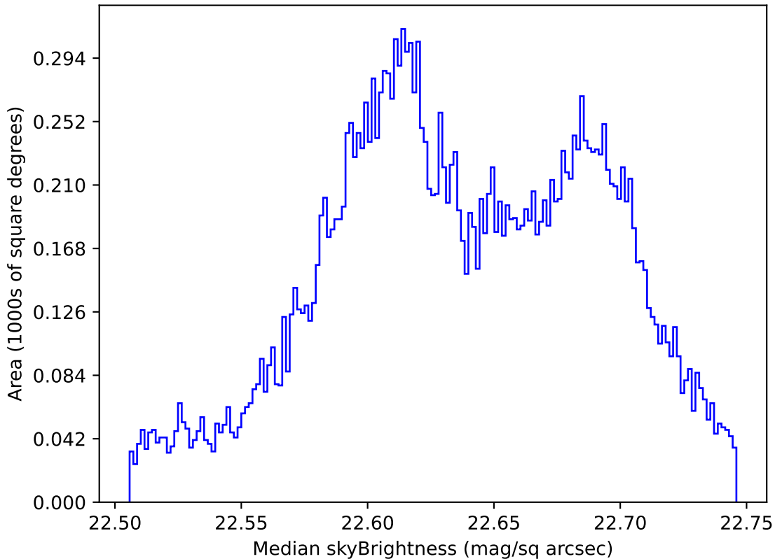
weather_cloudso6v3.4_10yrs All sky u band: Median skyBrightness
