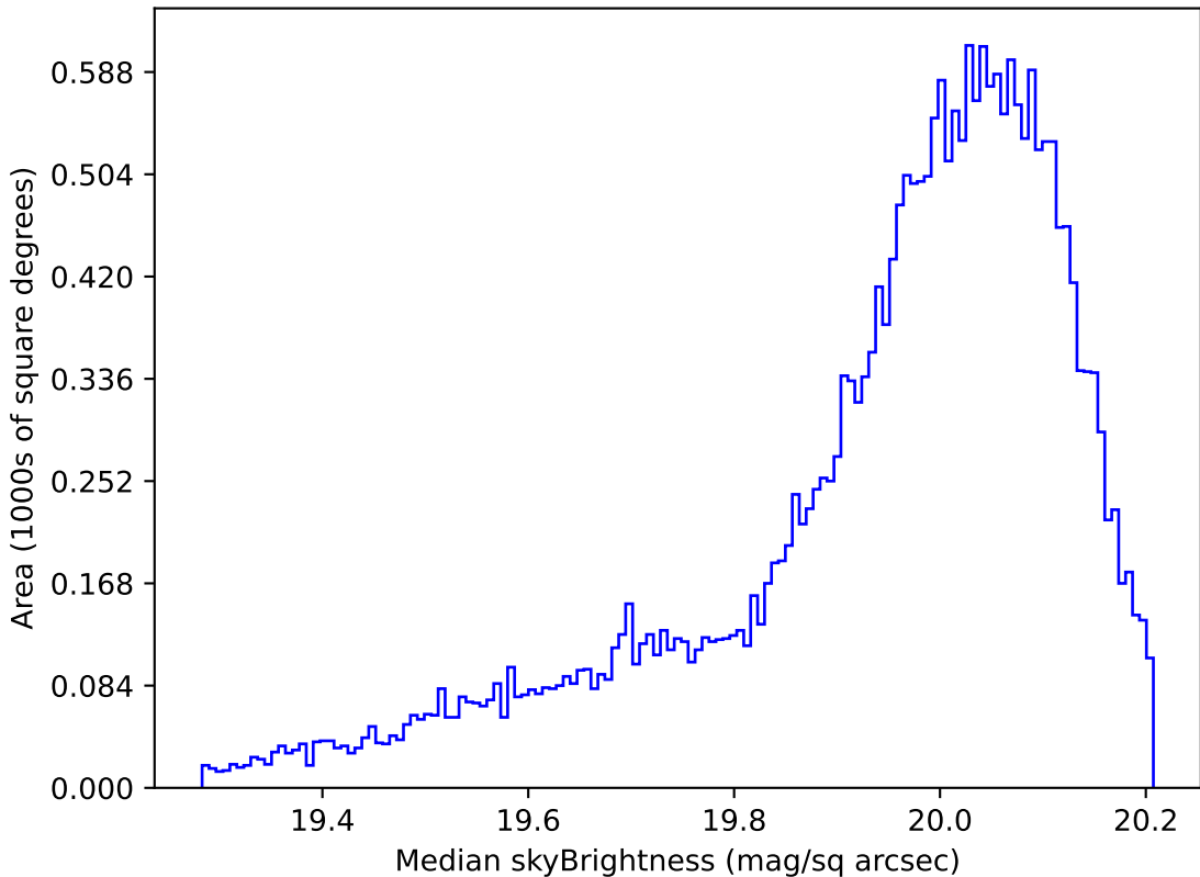
weather_cloudso6v3.4_10yrs All sky i band: Median skyBrightness
