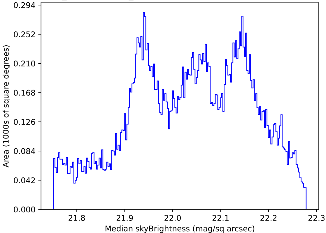
weather_cloudso6v3.4_10yrs All sky g band: Median skyBrightness
