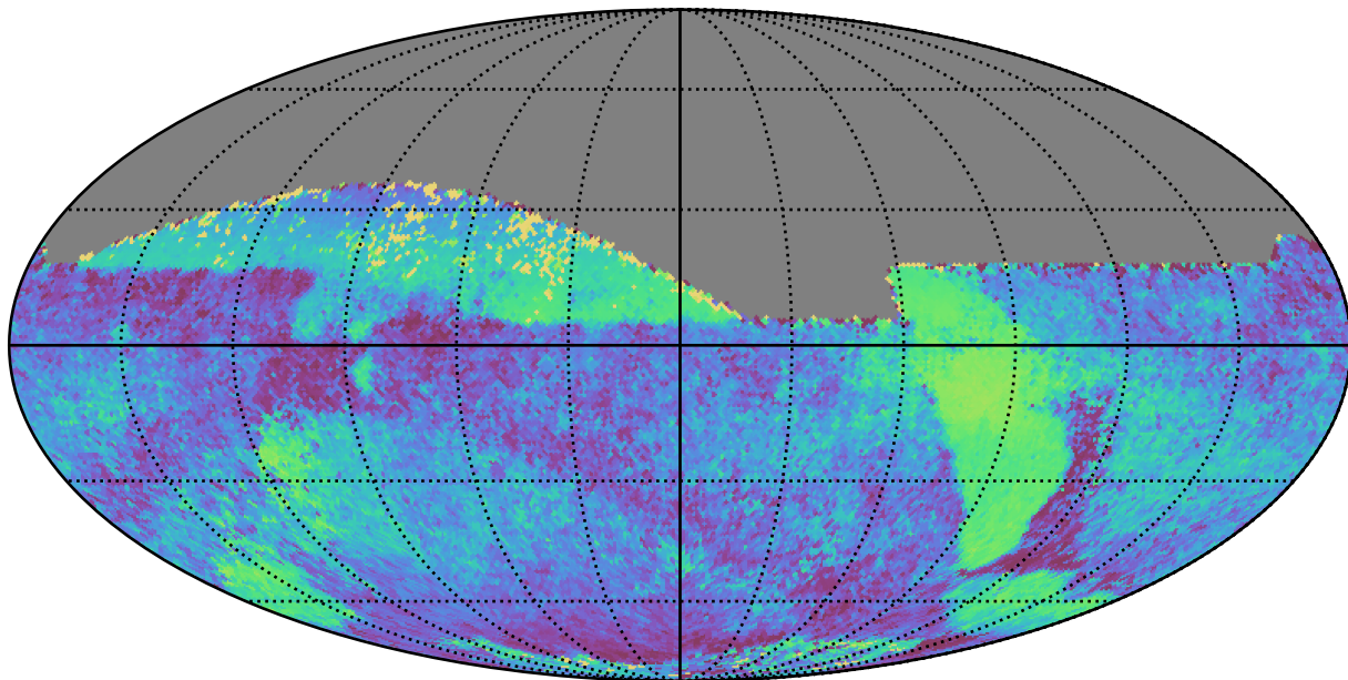
weather_cloudso6v3.4_10yrs All sky all bands: Median skyBrightness
