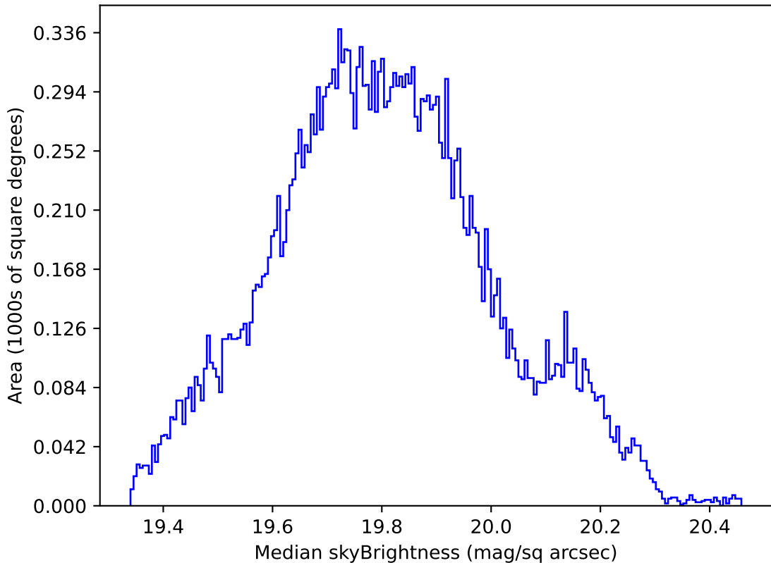
weather_cloudso6v3.4_10yrs All sky all bands: Median skyBrightness
