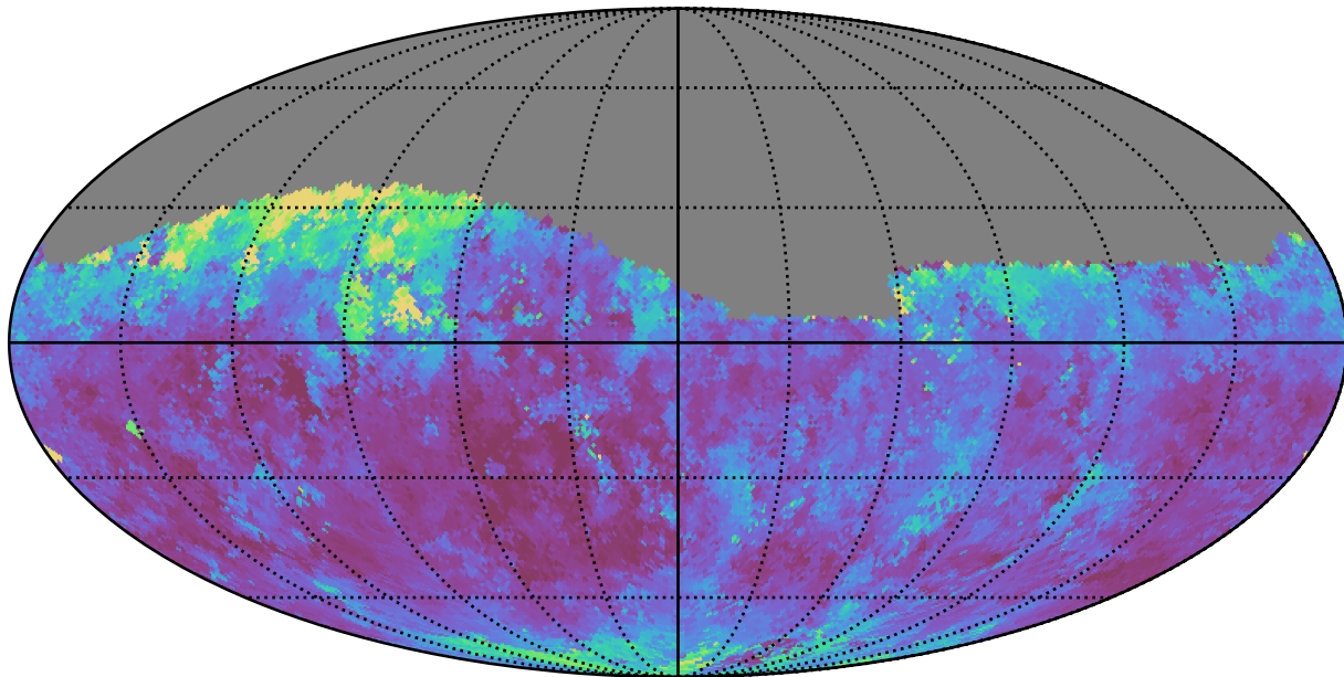
weather_cloudso6v3.4_10yrs Yr 1 z band: Median seeingGeom
